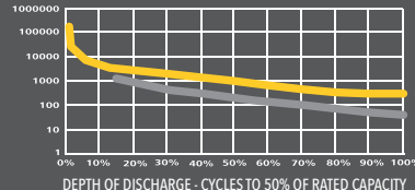
CYCLE LIFE VS. DEPTH OF DISCHARGE FOR OPTIMA BATTERIES
